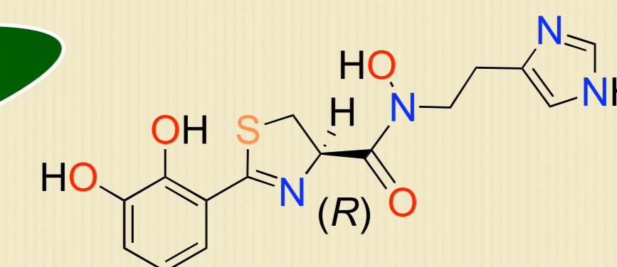
(-)-anguibactin
