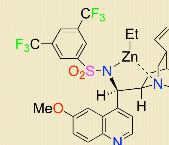
chiral sulfonamide-Zn complex catalyst
