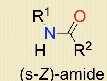
stereogenic P-atom
