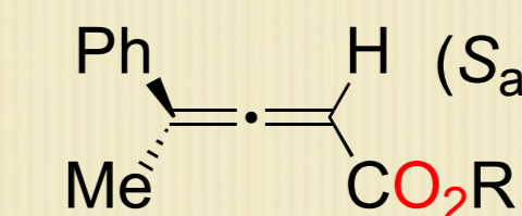
allene carboxylates
