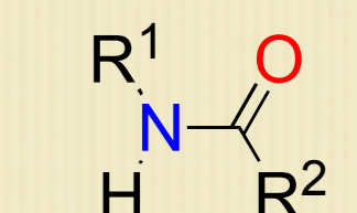
(s-Z)-amide
