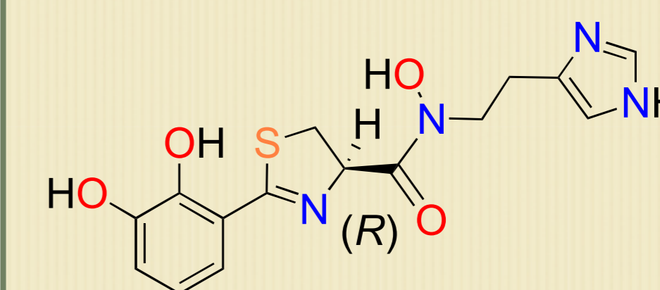
(-)-anguibactin
