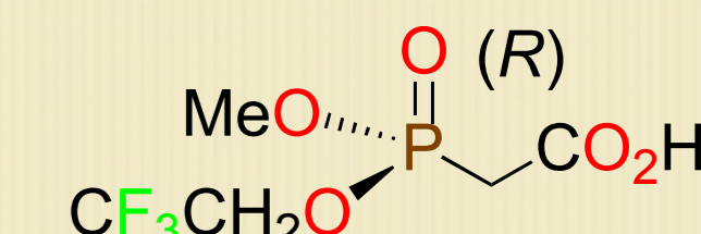
stereogenic P-atom
