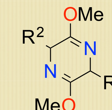
bis-lactim ether
