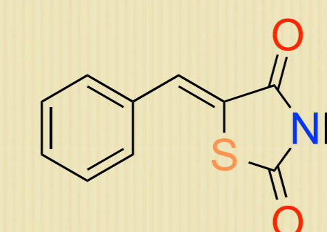
thiazolidine-2,4-dione
