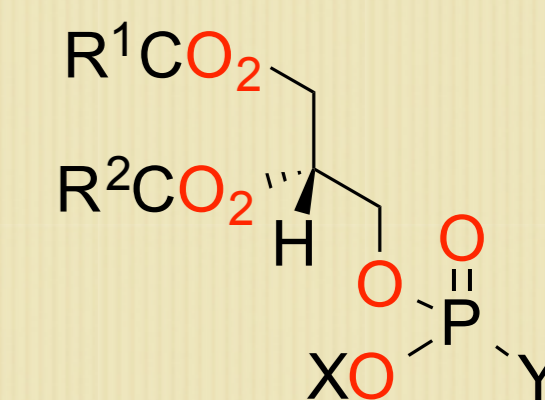
glycerophospholipid
