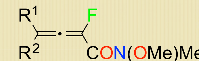
fluorinated allene
